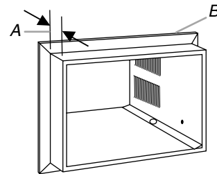
A. 1/2" (13 mm) extending into room B. Trim
