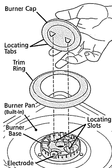
Standard and Power Burners
