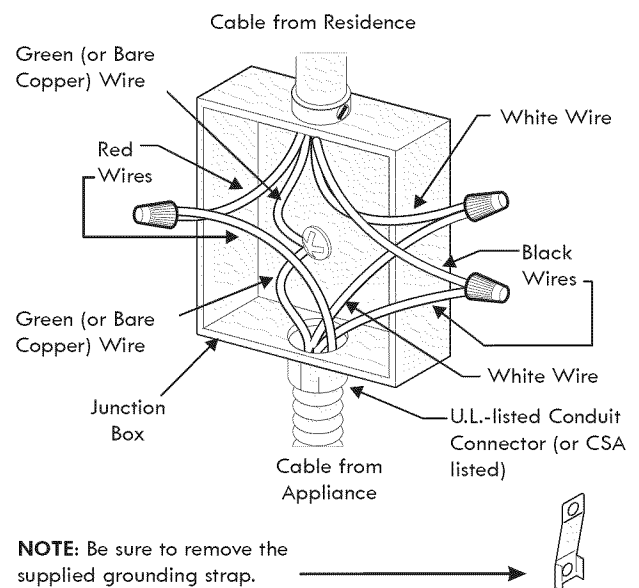
Figure 10 – 4-Wire Electrical System (Example: Junction Box)
