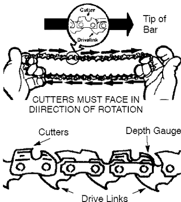
Drive Links
