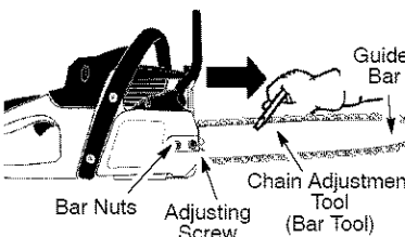
Adjusting Screw
