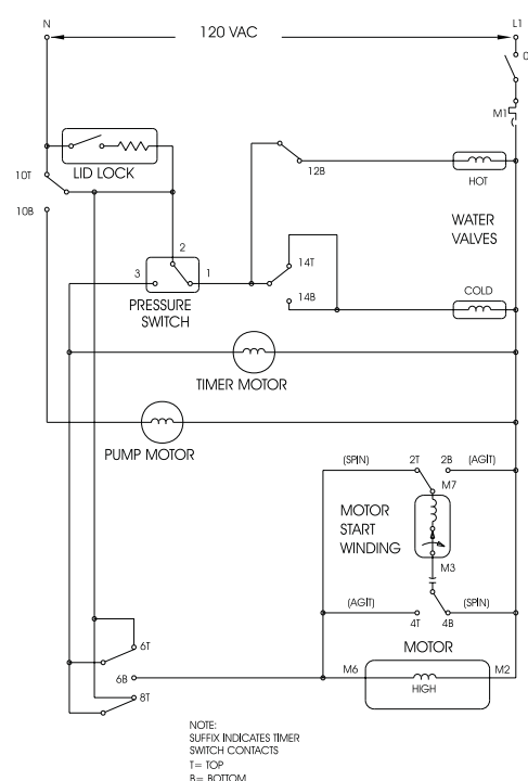
WIRING DIAGRAM P/N 131820700
