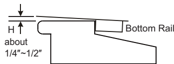
Wooden Window
