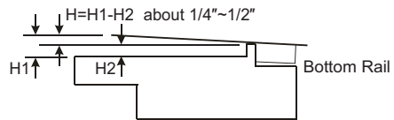
Vinyl-Clad Window
