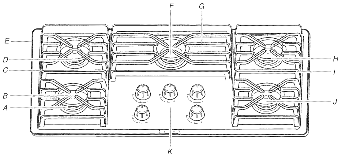
A. 17,000 BTU burner B. Surface burner cap C. Left surface burner grate D. 6,000 BTU burner
