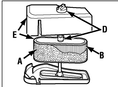
Figure 5-3: Briggs and Stratton air cleaner assembly.
