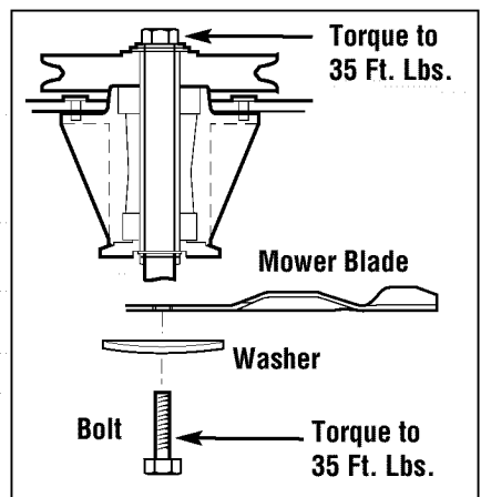
Figure 5-18: Blade spindle.
