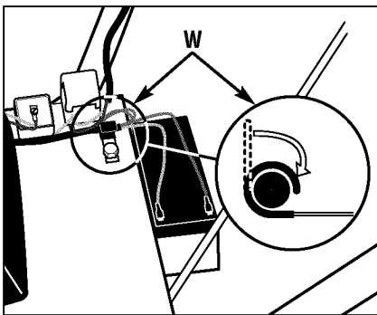
Figure 2-4: Attach wire harness with J-clips.
