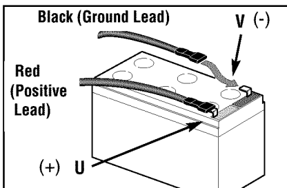
Figure 2-3: Connect wire terminals to battery terminals.
