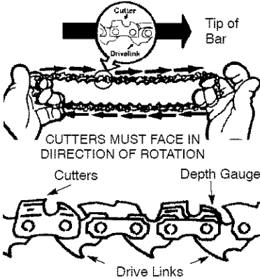
Drive Links
