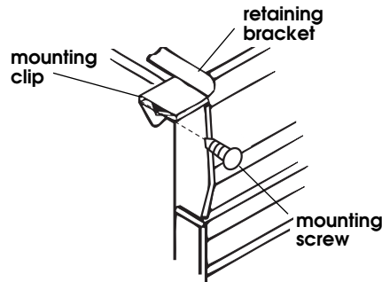
Cabinet-front mounting
