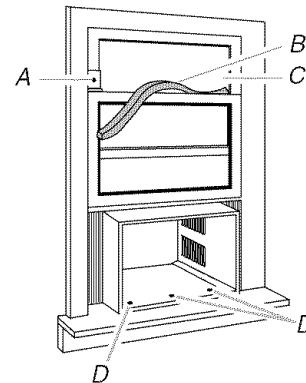
A. Window lock bracket B. Foam window sash seal C. Upper window glass D. #10 x \frac{1}{2} " pan-head Phillips screws (3)
