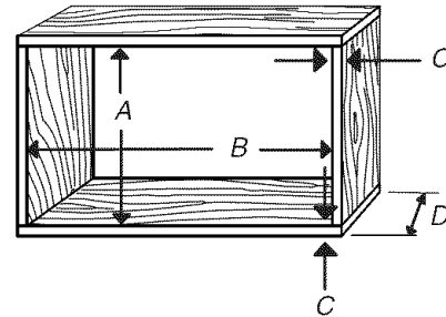
A. 16" (40.6 cm) C. Wood thickness B. 22⅝" (57.5 cm) D. Depth
