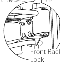
Hold the upper front rail and lower handles and push the rack all the way in until the install feature locks on the front support
