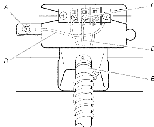
A. External ground conductor screw B. Neutral ground wire C. Center silver-colored terminal block screw D. Neutral wire (white or center wire) E. ¼" (1.9 cm) UL listed strain relief
