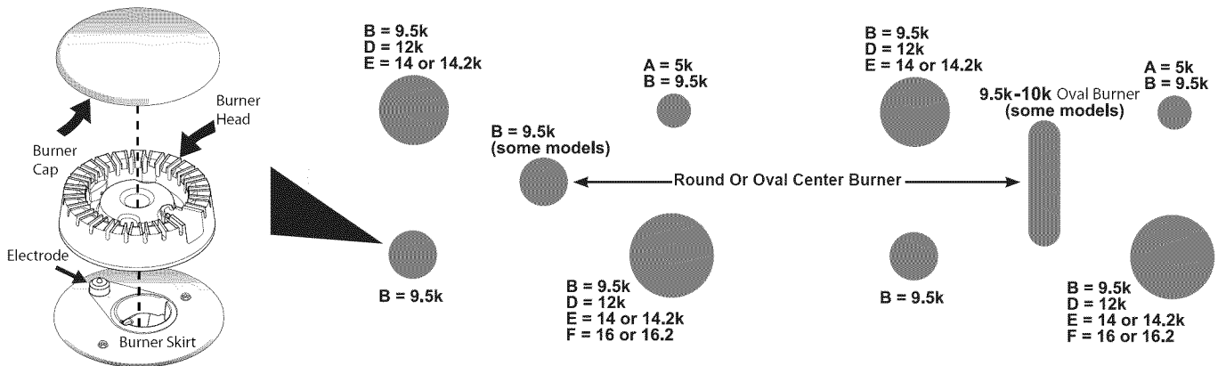
Example of Burner Assembly
