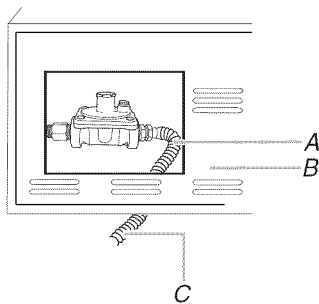
A. New CSA International approved “outdoor” flexible gas supply line B. Rear of grill C. To Natural gas or Local LP gas supply
