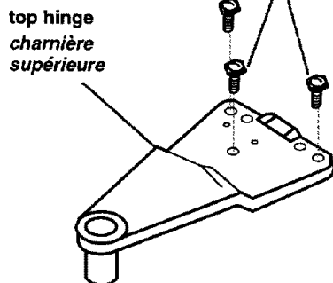
5/16" hex screws vis 5/16 po, tête hexagonale
