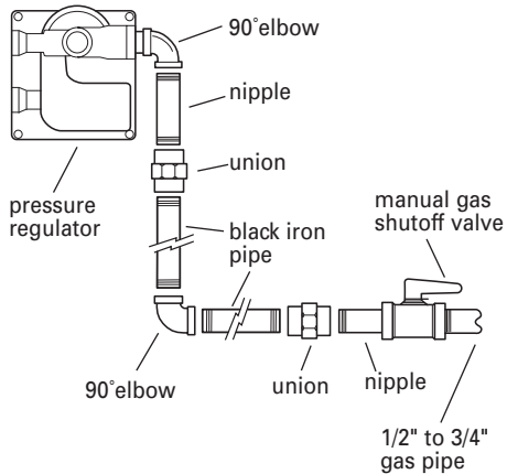
Typical rigid pipe connection
