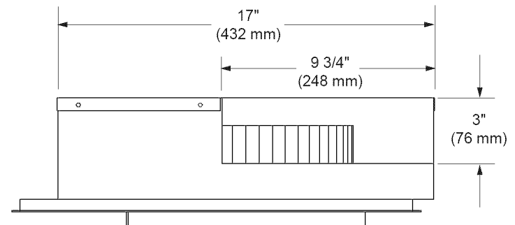
DUCT LOCATION SIDE VIEW
