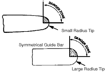
Reduced Kickback Symmetrical Guide Bar
