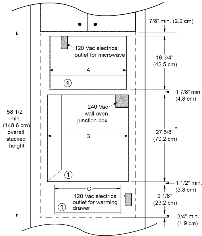
CUTOUT DIMENSIONS DMT2420/DMW2420 SHOWN
