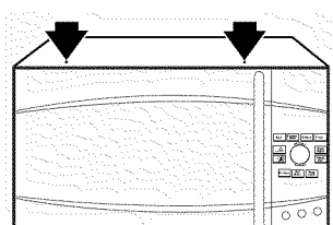
Remove 2 grille screws to remove the grille.
